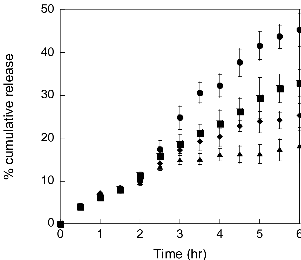
Figure 2 Triggered paclitaxel release was observed by incubating 10/90 (mol/mol) DMAEMA/HEMA nanoparticles crosslinked with 3 mol% TEGDMA for 2 hours at pH 7.4 (black triangle) followed by a reduction in pH to either 6.8 (black circle), 7.0 (black square), or 7.2 (black diamond) for 4 hours. The error is the standard deviation of the mean, where n = 3 [3].
